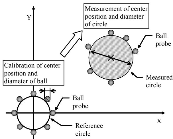
Fig. 2 Model for calibration of ball probe and measurement of circle in 2 dimensional area
