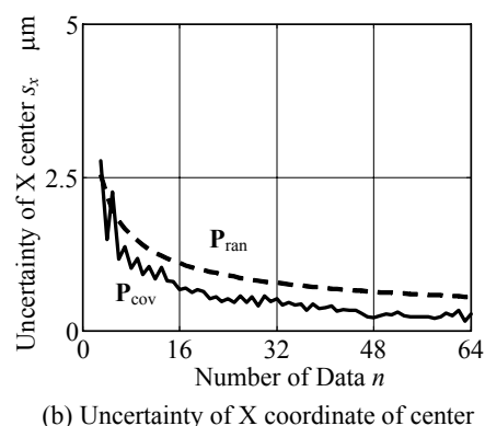
Fig. 7 Relationship between number of data n and uncertainty (standard deviation) of diameter s_d and X coordinate of center s_x
