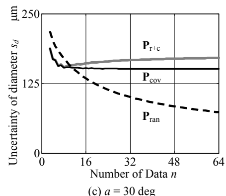
Fig. 9 Relationship between uncertainty of diameter s_d and number of data n in partial circle measurement of angle a = 180, 90 and 30 deg, by 3 calculated methods P_{r+c} , P_{cov} and P_{ran}
