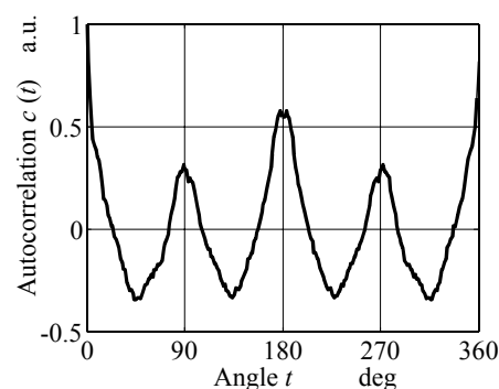
Fig. 6 Autocorrelation function of measured circle (Fig. 5 (b))
