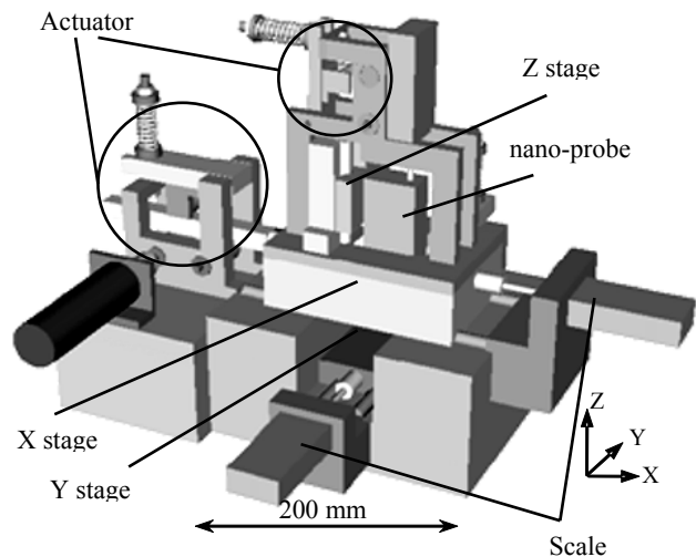
Fig. 2 Basic construction of Nano-CMM
