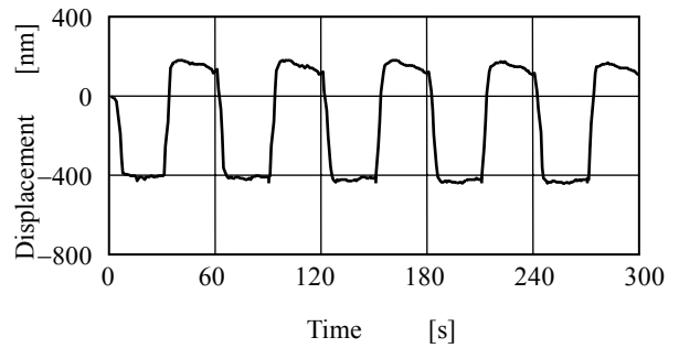
(a) Displacement of Y stage
