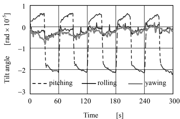
Fig. 9 Tilt angles (pitching, rolling and yawing) of X stage during 5 times of forward and backward movements
